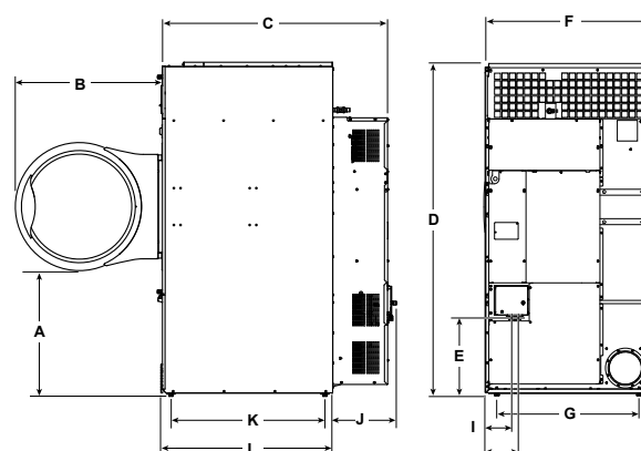
Right side
